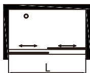
JD55 Flat Mutual Sliding with Pulley 平面窄边互移 下滑轮款 定制尺寸 / Custom size: L(1200-1800)xH2000mm
